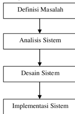
Gambar 2.1. Metode Waterfall
