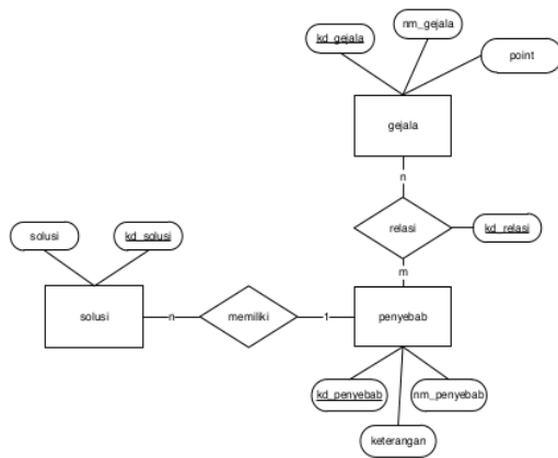
Gambar 5. Pemodelan Entity Relationship Diagram
