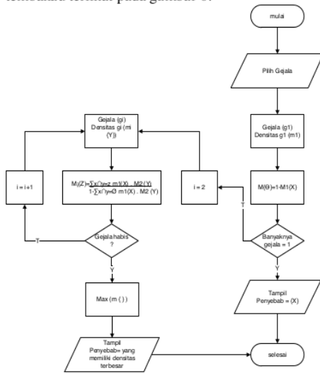
Gambar 6. Perancangan Flowchart Program
