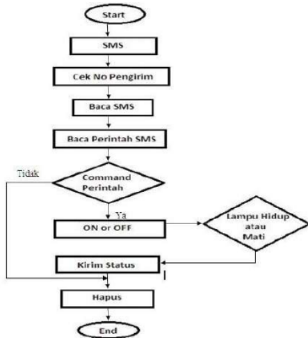
Gambar 2.3 Flowchart Kendali Lampu Rumah via SMS
