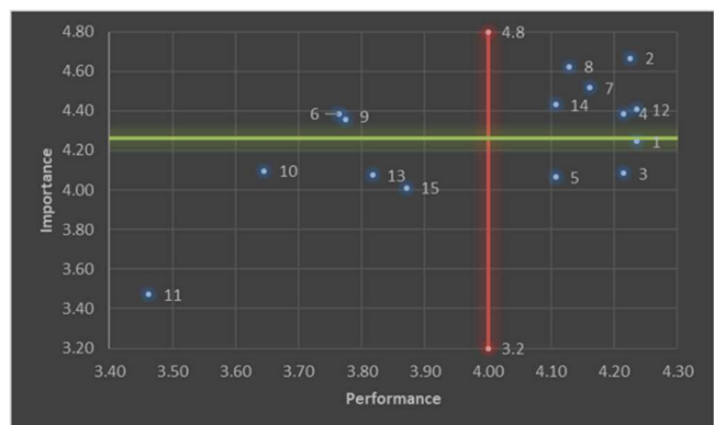
Gambar 2. Diagram Kartesius Analisis IPA TEFA Kebun Inovasi Polije
