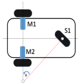
Figure 1. Robot drive system
