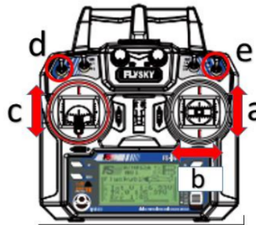
Figure 3. Remote channel mapping
