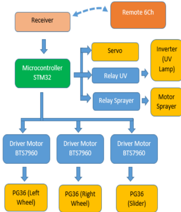
Figure 2. Block diagram system
