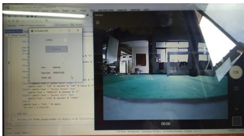
Figure 8 GUI view
