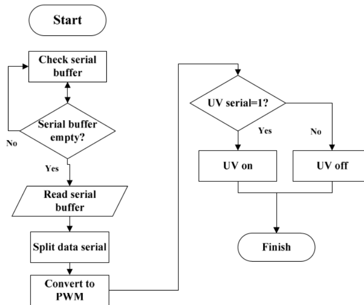
Figure 5 Flowchart System
