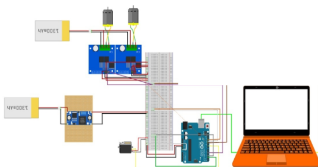
1 Figure 2. Diagram Block system
