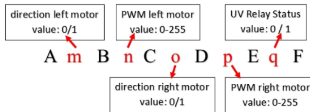
Figure 4. Data serial protocol
