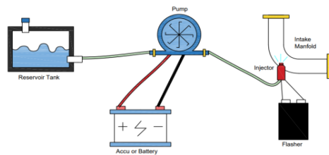
Gambar 4. Skema instalasi Water Injection System
