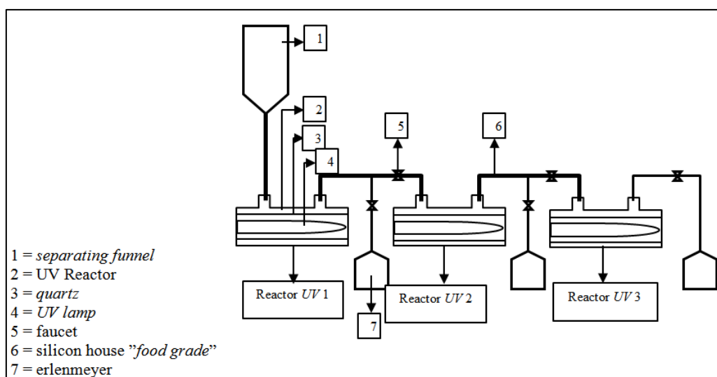
Figure 1. Serial system.
