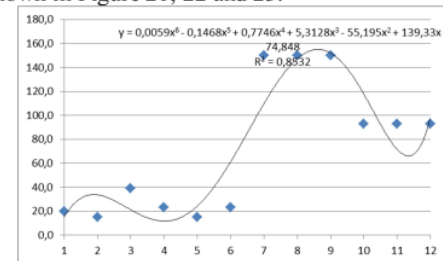
Figure 22. The pattern of distribution of Fecal coli for the period of January - December 2017 at the middle observation station.
