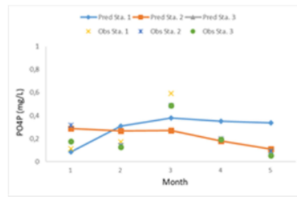
Figure 14. The Distribution Pattern of PO 4 P Observation and Prediction from the upstream to the downstream.
