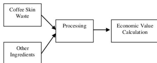
Fig. 1. Research Stages
