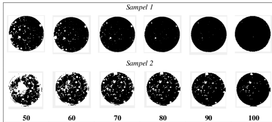
Gambar 11. Penentuan nilai ambang (T) proses Thresholding
