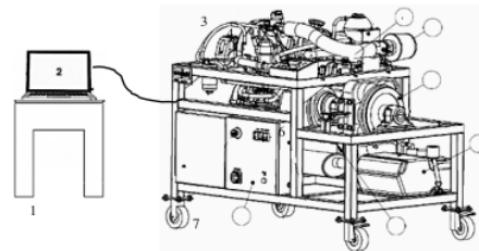
Gambar 3. Mesin Diesel Uji CM 12
