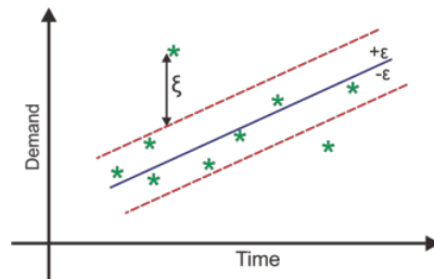
Gambar 3 Konsep Support Vector Regression (SVR)
