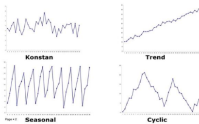
Gambar 2 Pola Data Time Series
