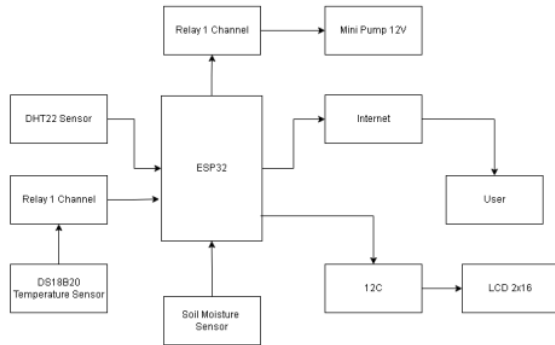
Fig. 2. Block diagram of portable smart SoC
