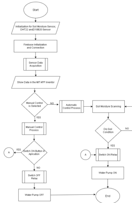
Fig. 3. Flowchart Portable Smart SoC
