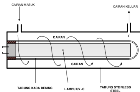
Gambar 5. UV Sterilizer
