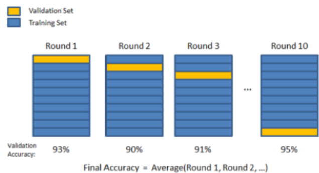
Figure 4. 10 fold Cross Validation Illustration
