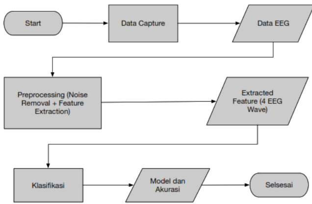
Figure 1. System Flowchart
