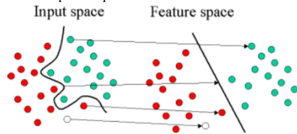
Figure 3. Hyperplane of Nonlinear SVM Illustration
