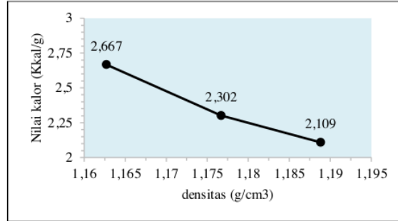
Gambar 6. Nilai Kalor vs densitas
