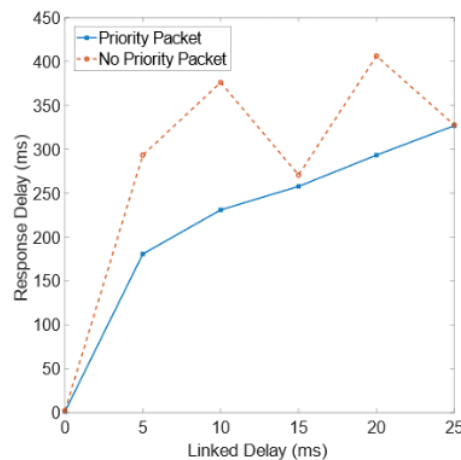
Gambar 4 Hasil Linked Delay
