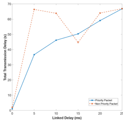
Gambar 5 Hasil Transmission Delay
