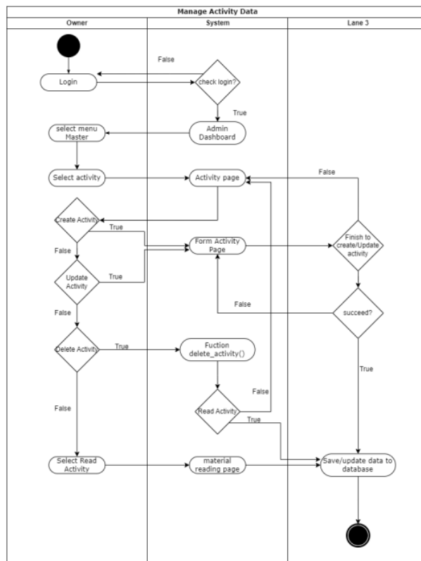
Figure 3. Activity diagrams manage activity data
