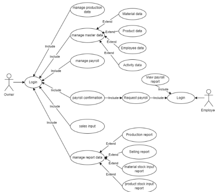
Figure 2. Use case management information system diagram
