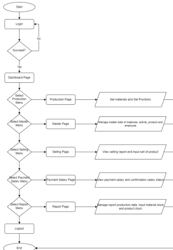
Figure 1. Flowchart management information system
