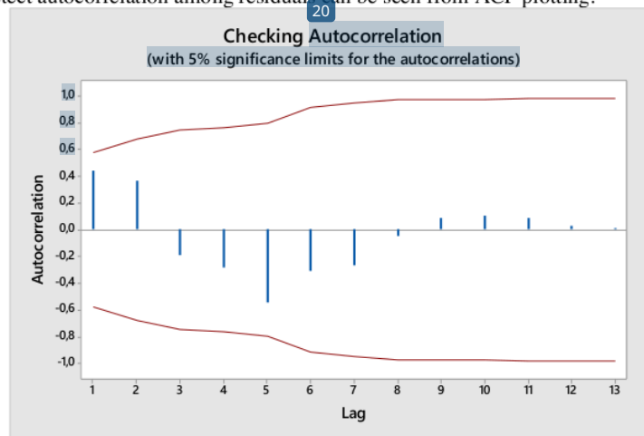
Figure 7. Autocorrelation Plot
