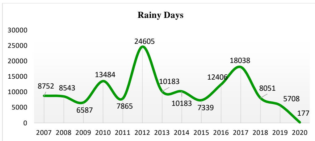
Figure 3. Rainy Days
