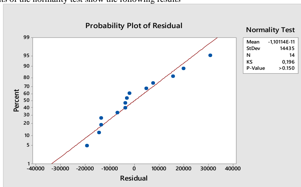
Figure 6. Normality Test
