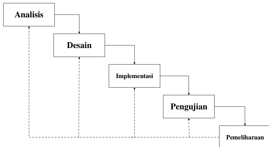
Gambar 1.4.1 Metode Waterfall
