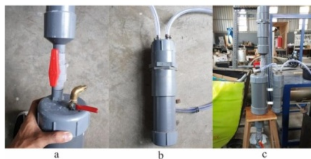
Fig. 6. Reservoir (a) inlet and outlet faucets; (b) bubbler; (c) the reservoir has been assembled.
