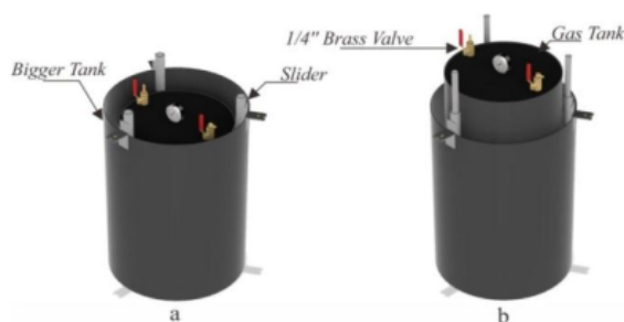
Fig. 3. Hydrogen gas storage tube design: (a) the tube sinks empty and (b) the tube floats when filled with gas.
