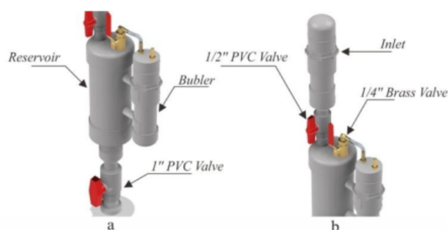
Fig. 2. Design of reservoir and bubler (a) and design of inlet (b).
