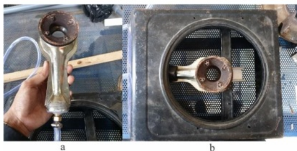
Fig. 8. Modified SNI 7368: 2007 stove, (a) burner modification, (b) modified stove.
