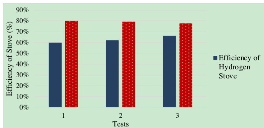
Fig. 13. The comparison of stove efficiency with hydrogen and LPG fuels.
