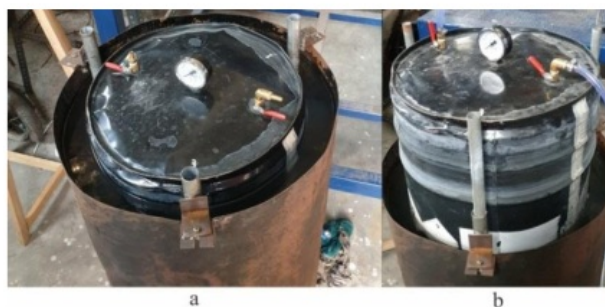
Fig. 7. Hydrogen gas storage tubes (a) the tubes sink empty; (b) the tube floats when filled with gas.
