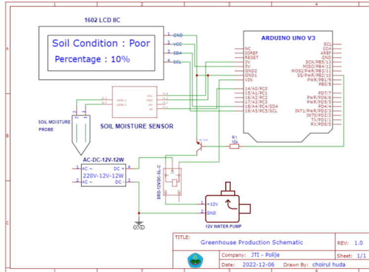
Fig. 1 Schematic diagram of the IoT devices
