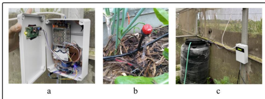
Fig. 4 The implementation of IoT devices inside greenhouse production: (a) the IoT box; (b) soil moisture sensor placement; (c) water reservoir and pump placement
