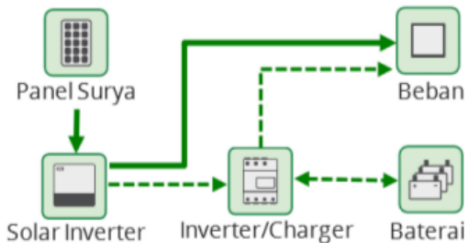
Gambar 4.7 Skema Sistem Off-Grid
