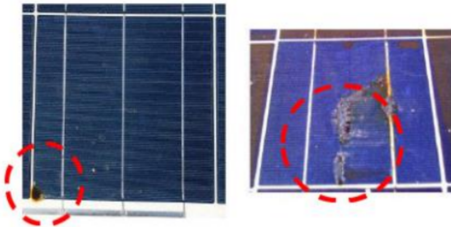
Gambar 5.13 Panel Surya Hotspot (Sumber: USAID)
