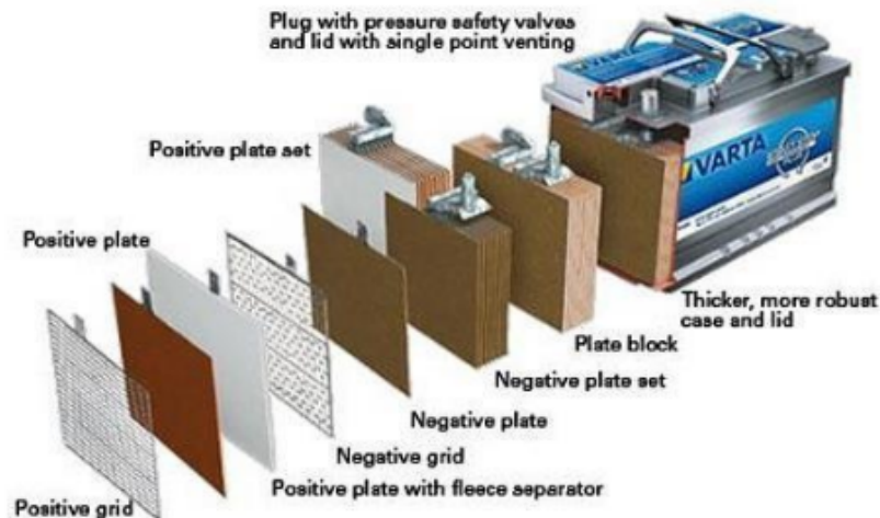
Gambar 3.13 Gambar Baterai AGM ( Absorbent Glass Matt ) (sumber: offgridham.com )
