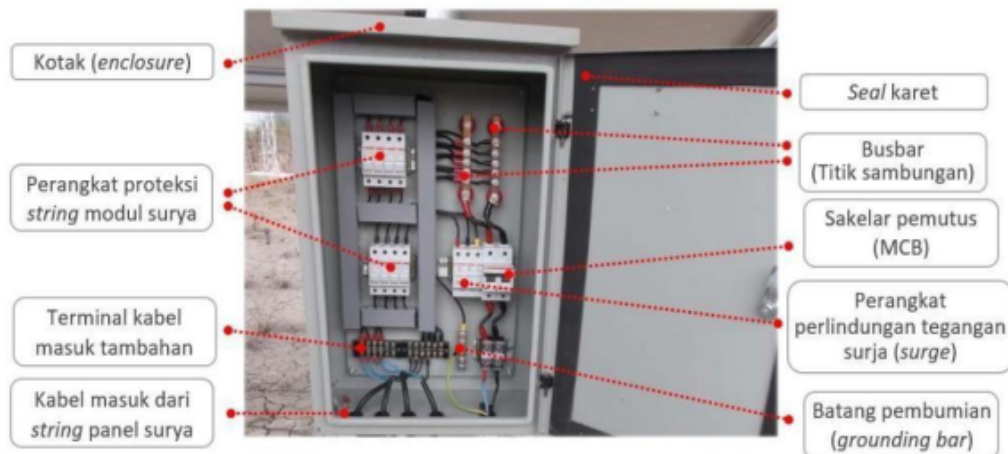
Gambar 3.15 Gambar Combiner Box (sumber: energypedia.info )
