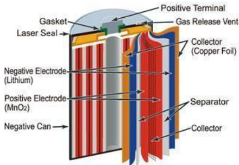
Gambar 3.14 Gambar Baterai Lithium-ion
