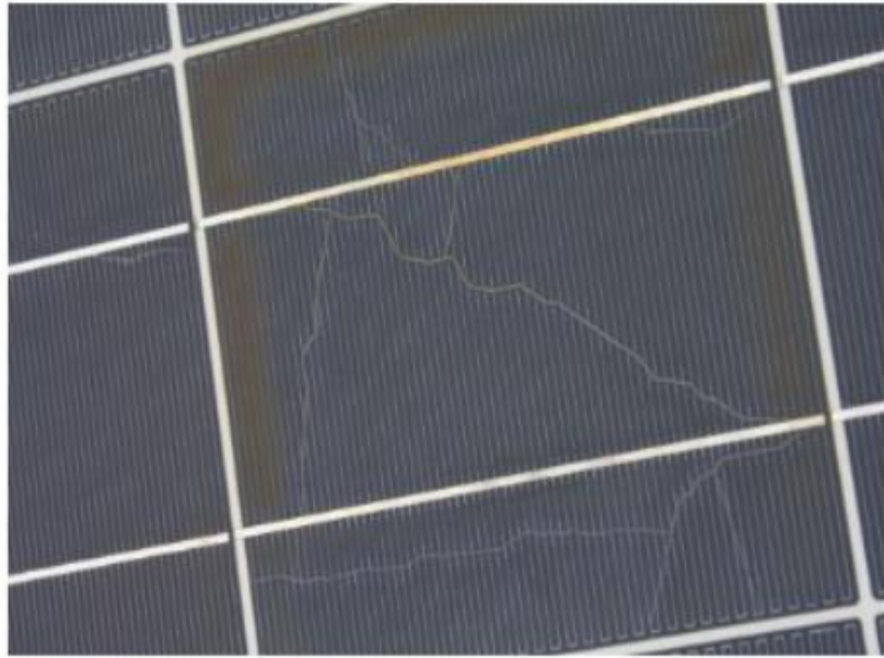
Gambar 4.19 Snail Track (Sumber: ica solar)
