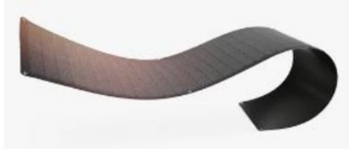
Gambar 2.8 Panel Surya Thin Film CIGS (Sumber: Google Images)
