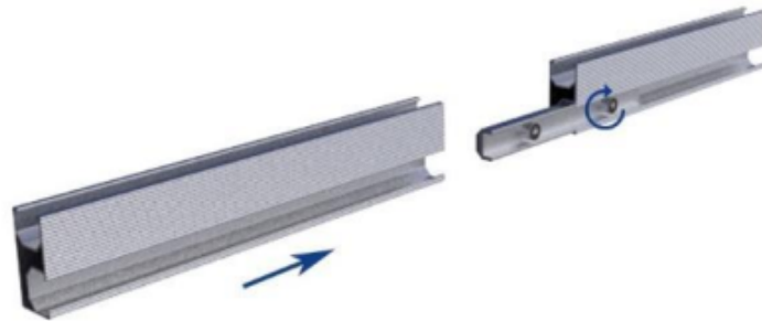
Gambar 4. 17 Gambar joint rail (Sumber: Solarrex.com)
