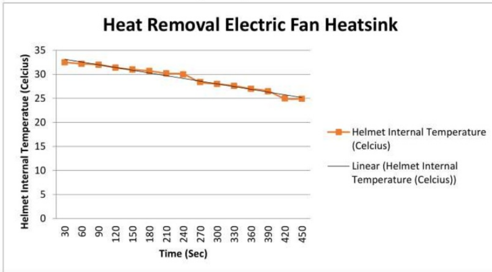
Figure 3. Heat removal electric fan heatsink
