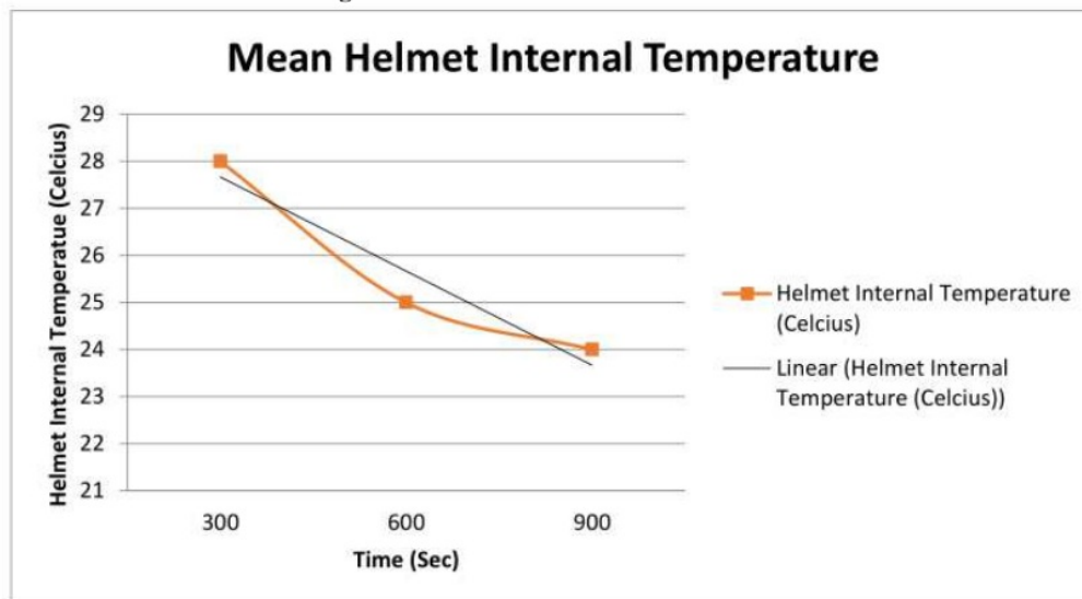
Figure 4. Mean helmet internal temp.
