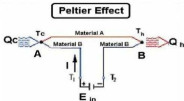
Figure 1. Peltier Effect
