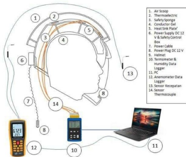
Figure 2. The apparatus setting of active passive thermoelectric system helmet
