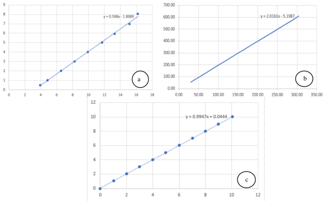
Figure 5. Calibration data for ACS712 30A Sensor (a), Irradiation Sensor (b), and Voltage Sensor (c).
