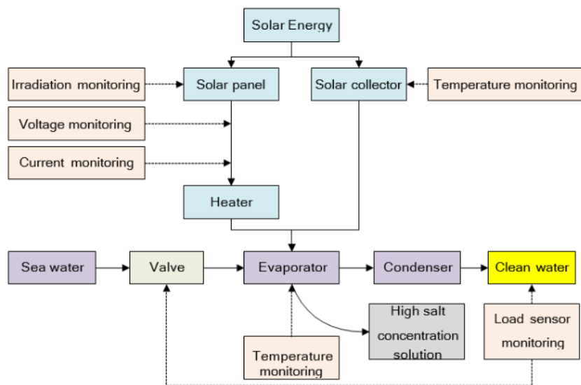
Figure 1. Seawater distillation proposed system.
