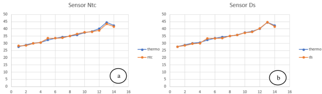
Figure 6. Calibration data for NTC sensor (a) and Ds18b20 Sensor (b).
