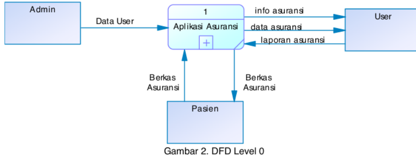
Gambar 2. DFD Level 0
