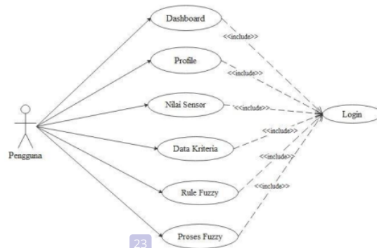
Gambar 4. Use Case
