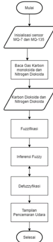
Gambar 3. Flowchart System
