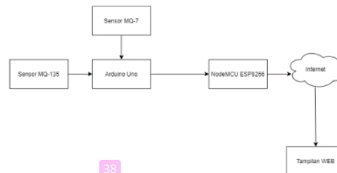
Gambar 2. Blok Diagram
