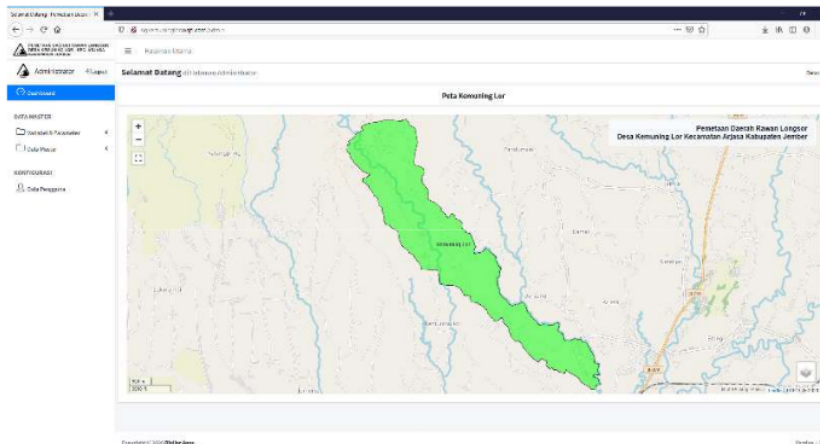
Figure 10. Administrator Page
