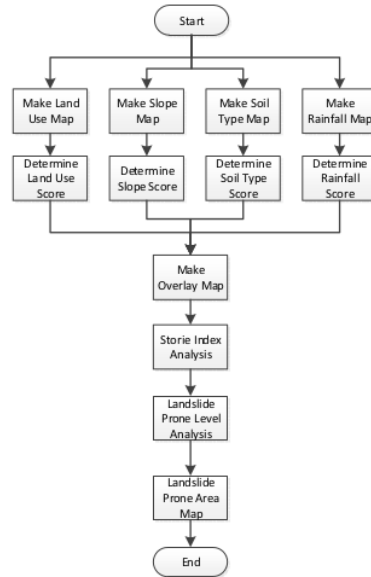
Figure 1 Research method
