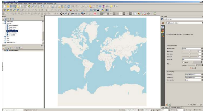
Figure 3. Quantum GIS
