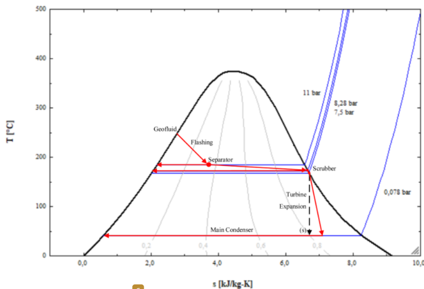
Fig. 3. Temperature-Entropy (T-s) Diagram
