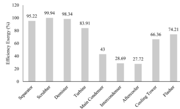
Fig. 6. Exergetic Efficiency of Each Component
