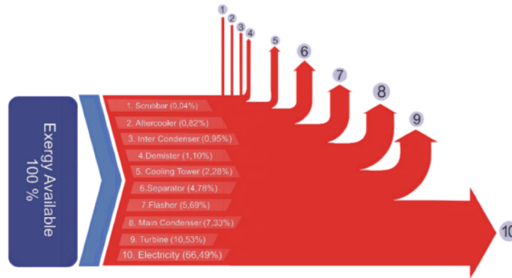
Fig. 7. Sankey Diagram of exergy flow
