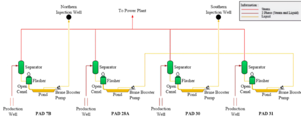
Fig. 2. Gathering System of Dieng geothermal power plant
