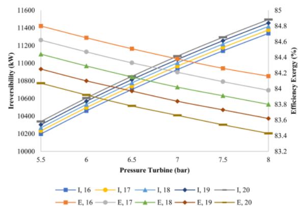
Fig. 8. Effect of Pressure on Irreversibility and Exergetic Efficiency
