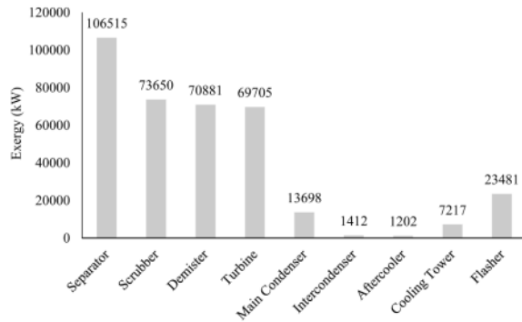
Fig. 4. Total Exergy of Each Component
