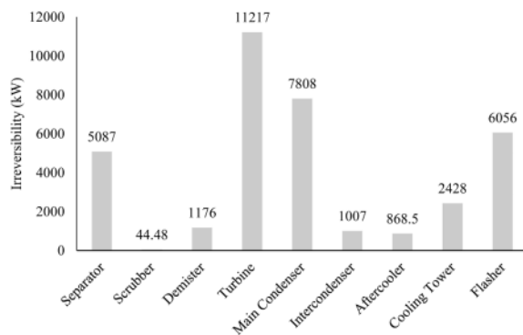
Fig. 5. Irreversibility of Each Component
