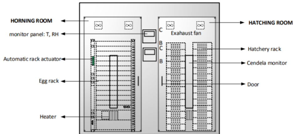
Figure 1. Duck egg hatcher with automatic system
