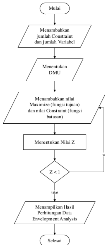
Gambar 1. Flowchart Sistem
