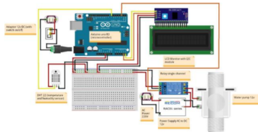
Gambar 2. Prototype Alat ACoSy
