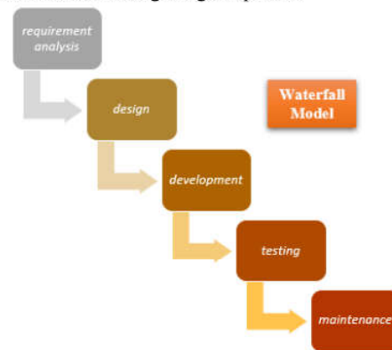
Gambar 1. Waterfall Model
