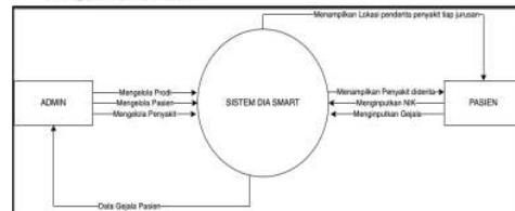
Gambar 4. DFD Level 0
