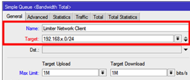
Figure 4. PCQ Queue
