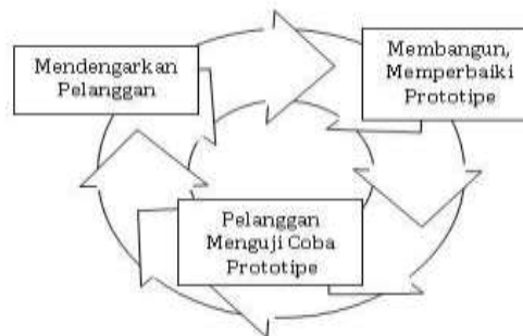
Gambar 1.2 Metode Prototype
