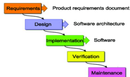
Gambar 1. Metode Waterfall
