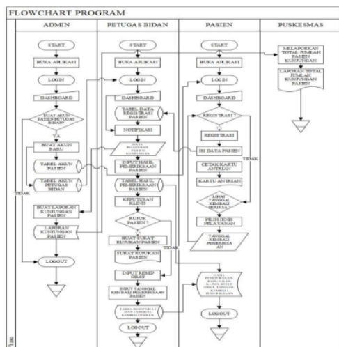
Gambar 2. Flowchart Program
