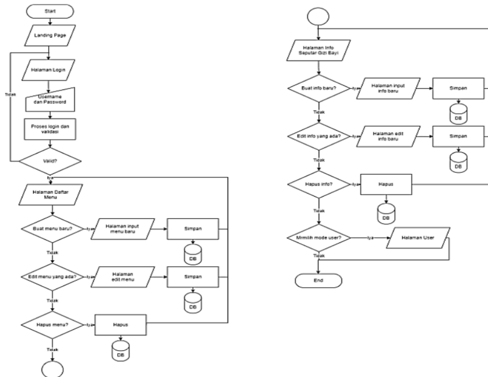
Gambar 2. Flowchart sistem admin
