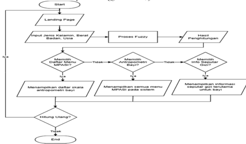
Gambar 1. Flowchart sistem user
