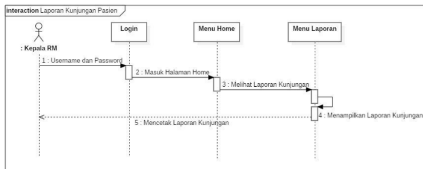
Gambar 8. Sequence Diagram Laporan Kunjungan
