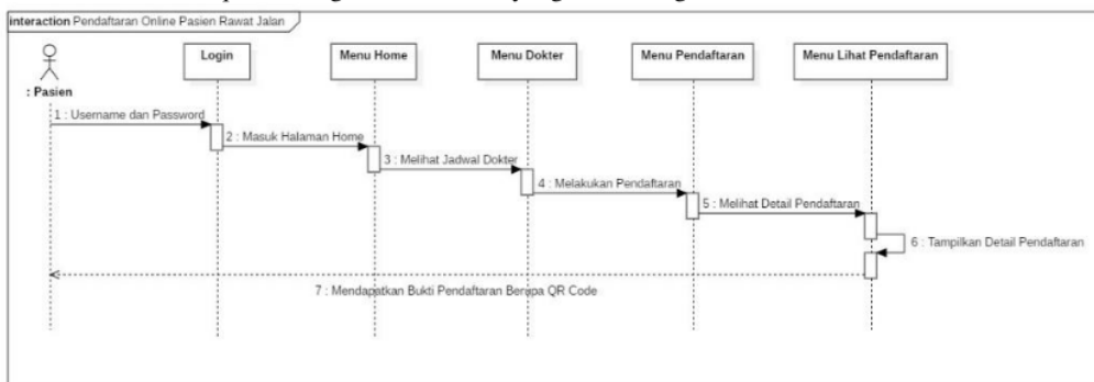
Gambar 6. Sequence Diagram Mendaftar Online
