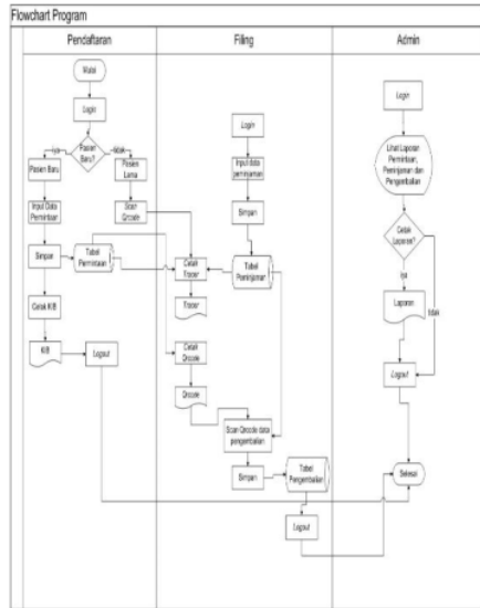
Gambar 4. Flowchart Program
