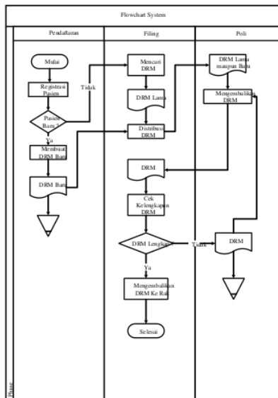
Gambar 3. Flowchart System
