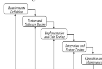
Gambar 2. Metode Waterfall
