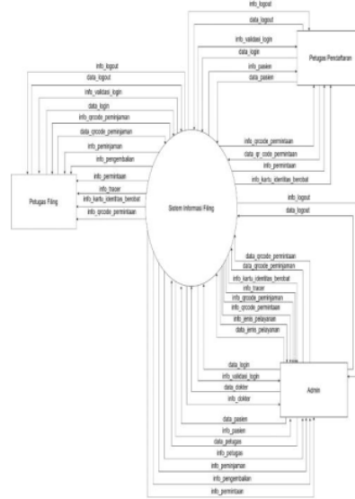
Gambar 5. Context Diagram/Diagram Level 0
