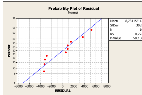
Figure 1. Normality test of Residual
