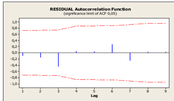
Figure 2. ACF Residual of Regression Model
