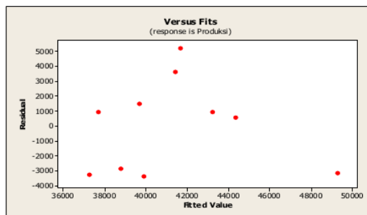
Figure 3. Scatter plot Residual and Production
