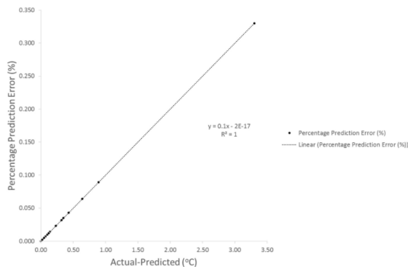
Fig. 8. Regression percentage prediction error of temperature.
