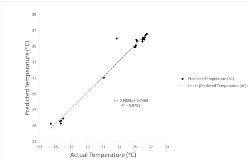
Fig. 6. Regression of actual temperature and predicted temperature.
