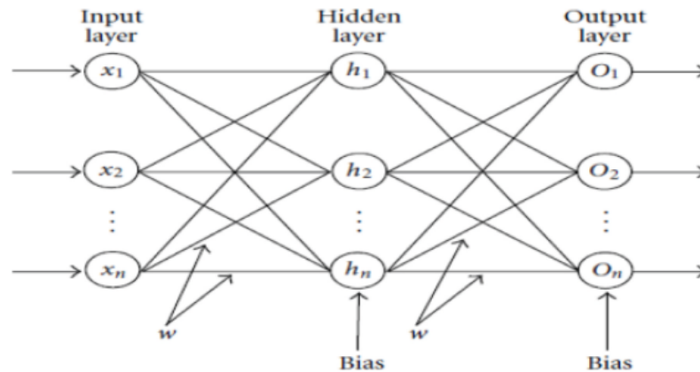
Fig. 3. Backpropagation Algorithm Artificial Neural Network Architecture [32].
