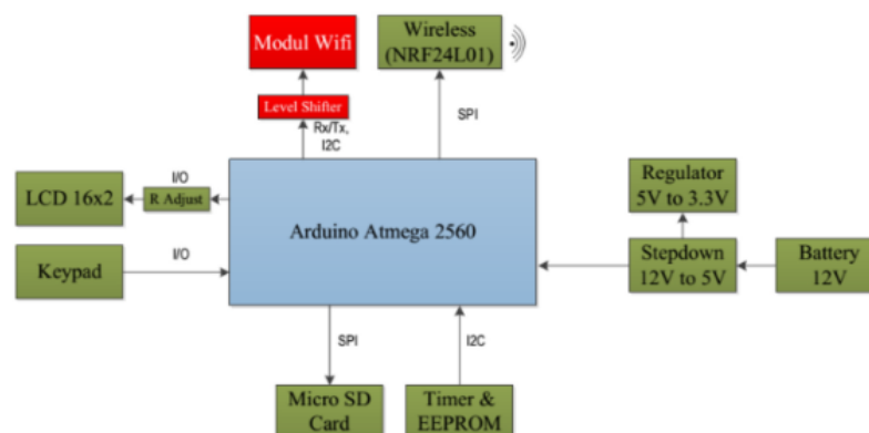
Fig. 1. Main master diagram.
