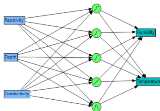
Fig. 4. Schematic of the ANN diagram used.
