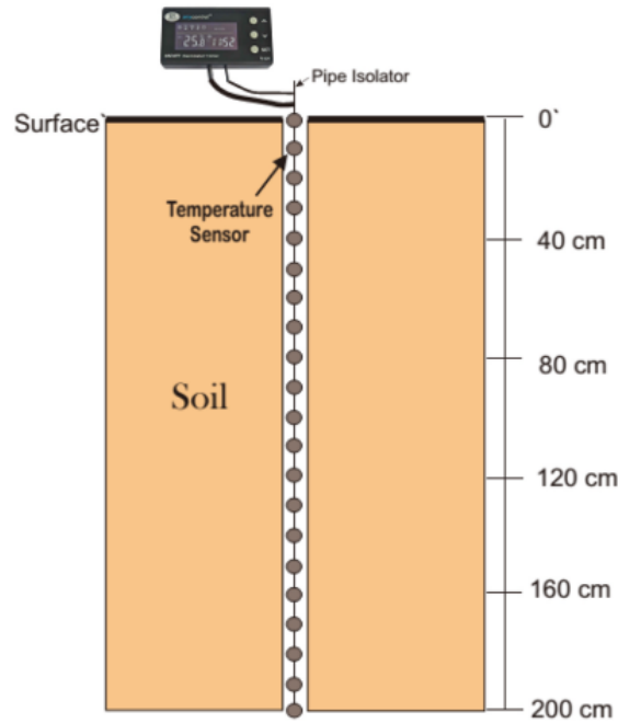
Fig. 2. Temperature measurement position.
