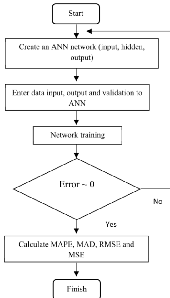
Fig. 5. Flowchart of research.
