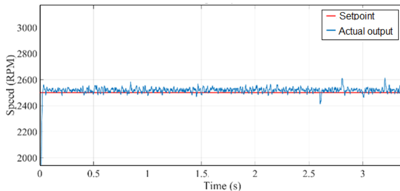
Fig. 17 - ANFIS response system in scenario 2
