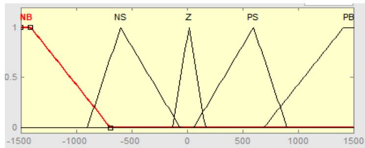
Fig. 4 - Membership input error
