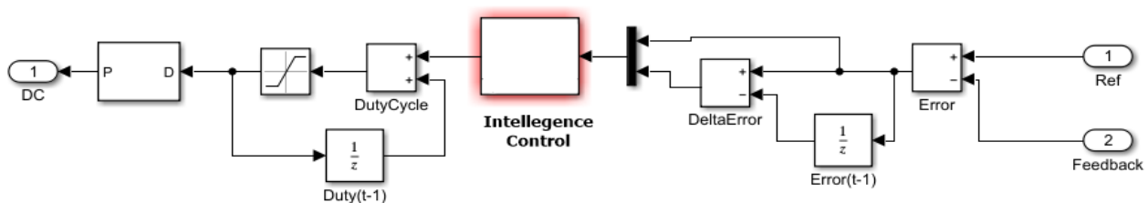
Fig. 3 - Control block design in detail
