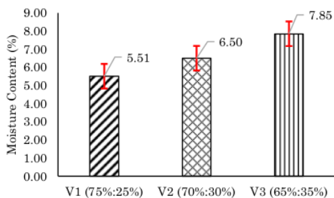
Fig. 3 Moisture content of coconut shell briquettes with cassava peel adhesive
