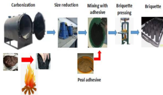
Fig. 1 Briquette preparation schematic diagram
