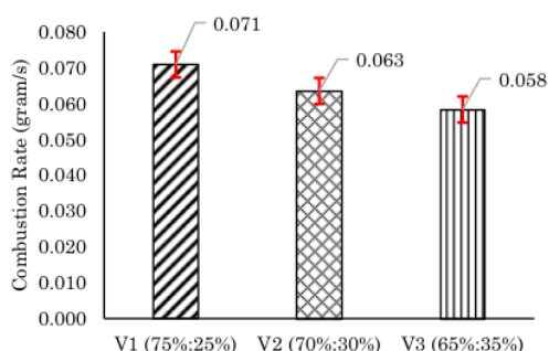
Fig. 5 Combustion rate of coconut shell briquettes with cassava peel adhesive
