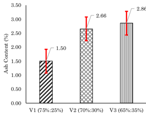
Fig. 4 Ash content of coconut shell briquettes with cassava peel adhesive
