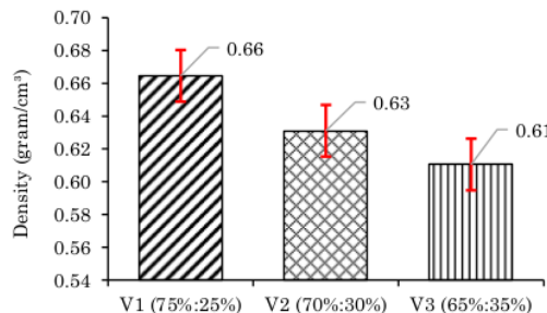
Fig. 2 Density of coconut shell briquettes with cassava peel adhesive
