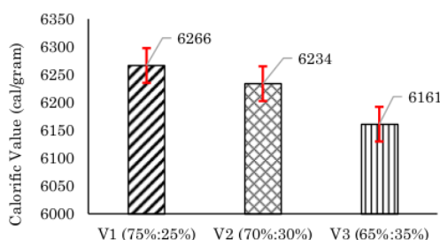
Fig. 6 Calorific value of coconut shell briquettes with cassava peel adhesive
