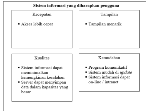
Gambar 4. Diagram afinitas
