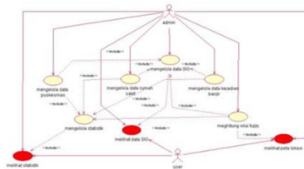
Gambar 7 Use case diagram
