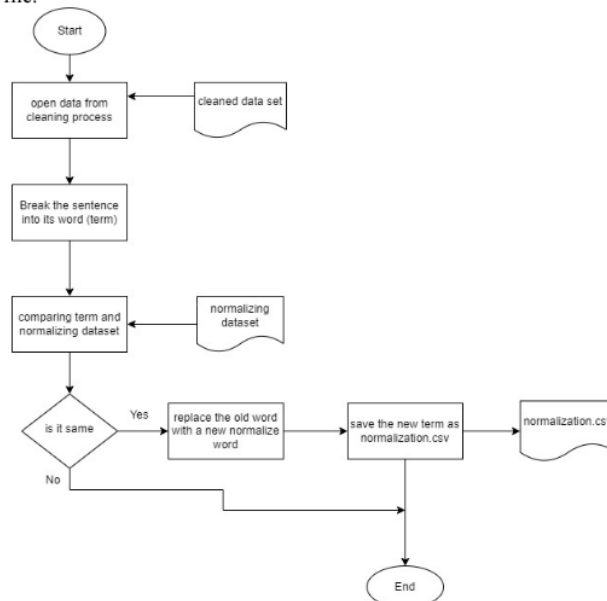
Figure 2. Term normalizing flowchart
