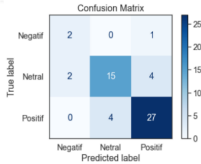
Figure 3. Confusion Matrix
