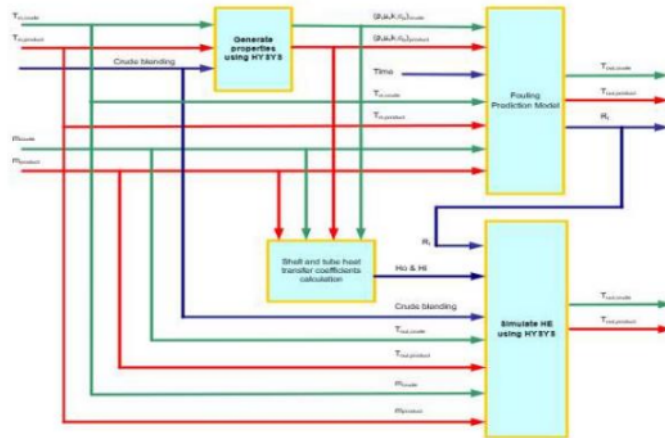
Figure 3. Schematic diagram of integrated model
