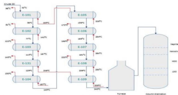
Figure 1. The schematic diagram of the CPTAFAF
