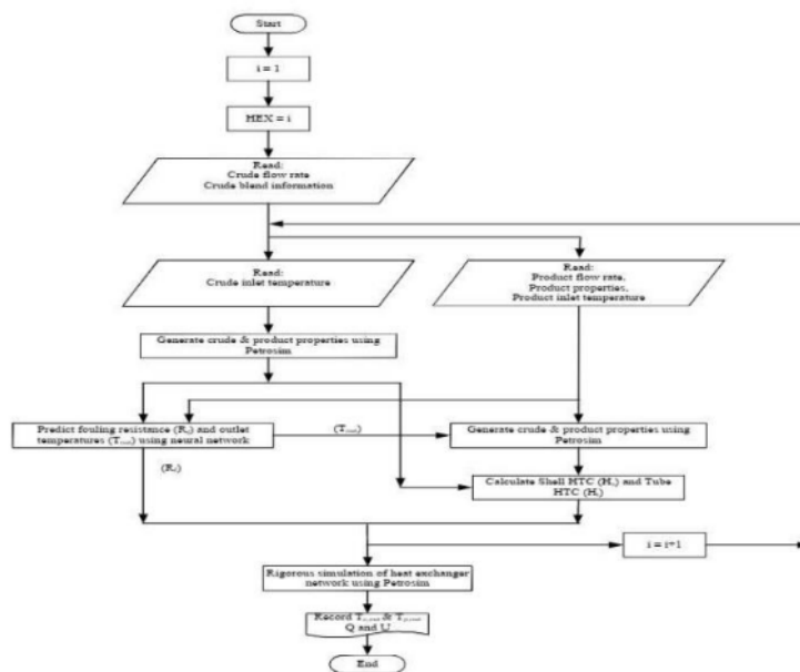
Figure 4. Flowchart of integrated models software
