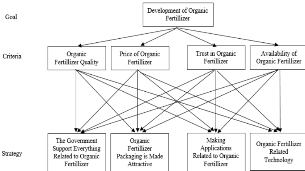
Figure 2. Hierarchy diagram
