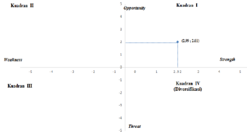
Figure 1. SWOT diagram
